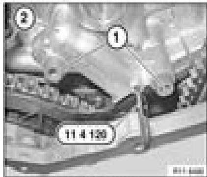
Fig. 76. Removing Chain Tensioner
