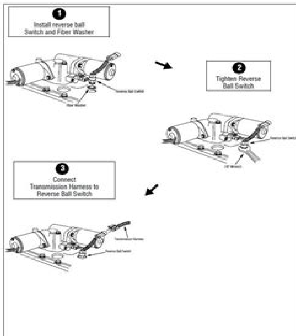
Reverse Ball Switch Installation
