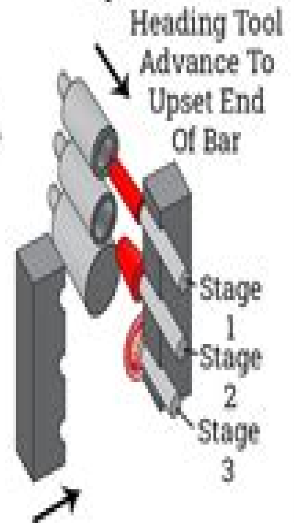
Upset
