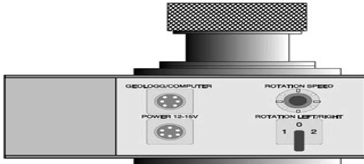
Front Panel of Instrument Head of the Electrical Vane Test Apparatus EVT 2000
