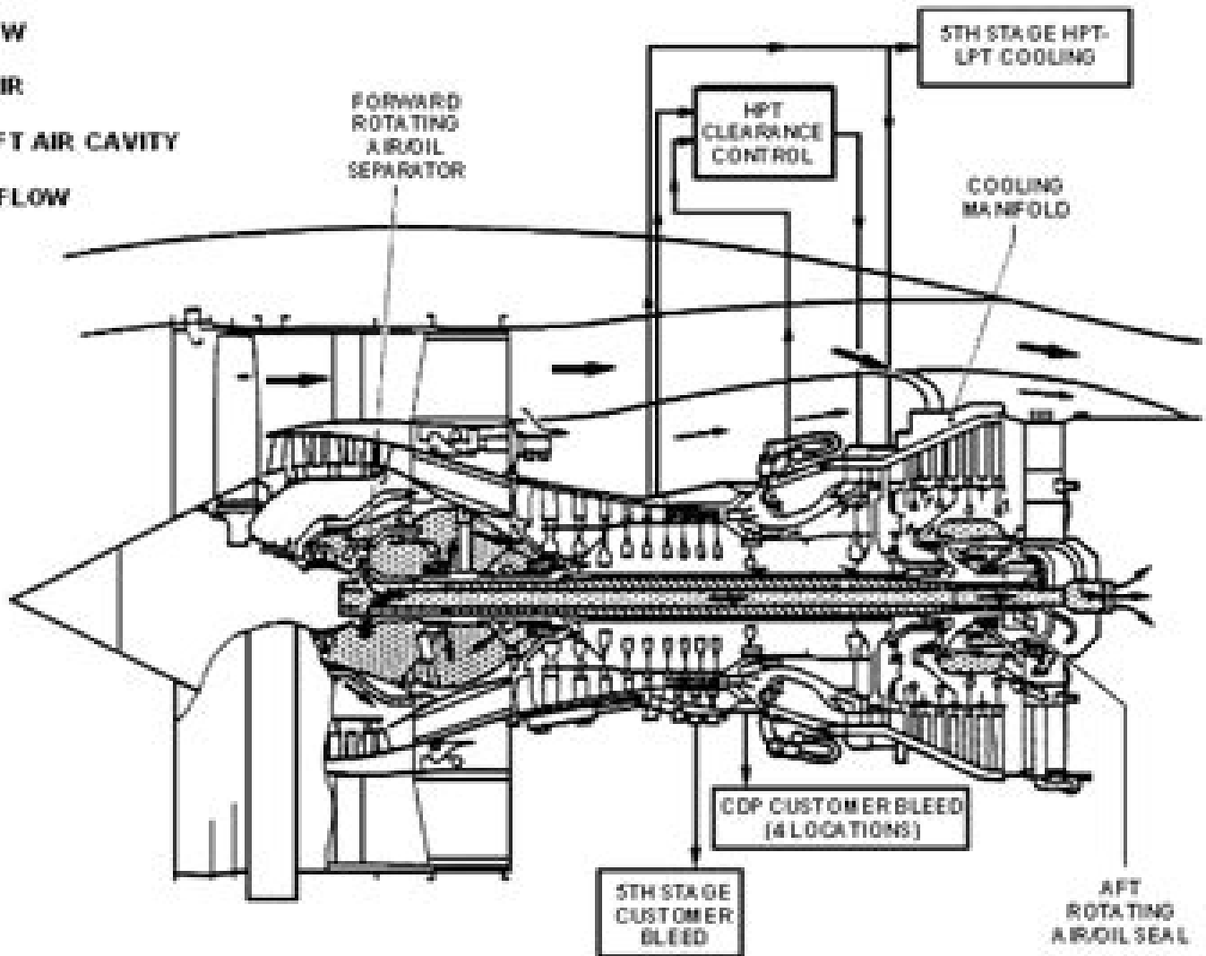
AIR SYSTEM SCHEMATIC
