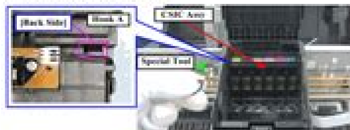
Figure 4-48. Removing the CSIC Assy (1)
