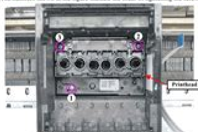
Figure 4-51. Removing the Printhead (1)
