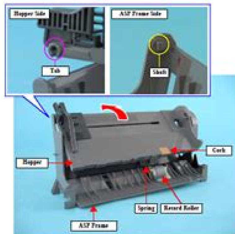
Figure 4-7. Removing Hopper
