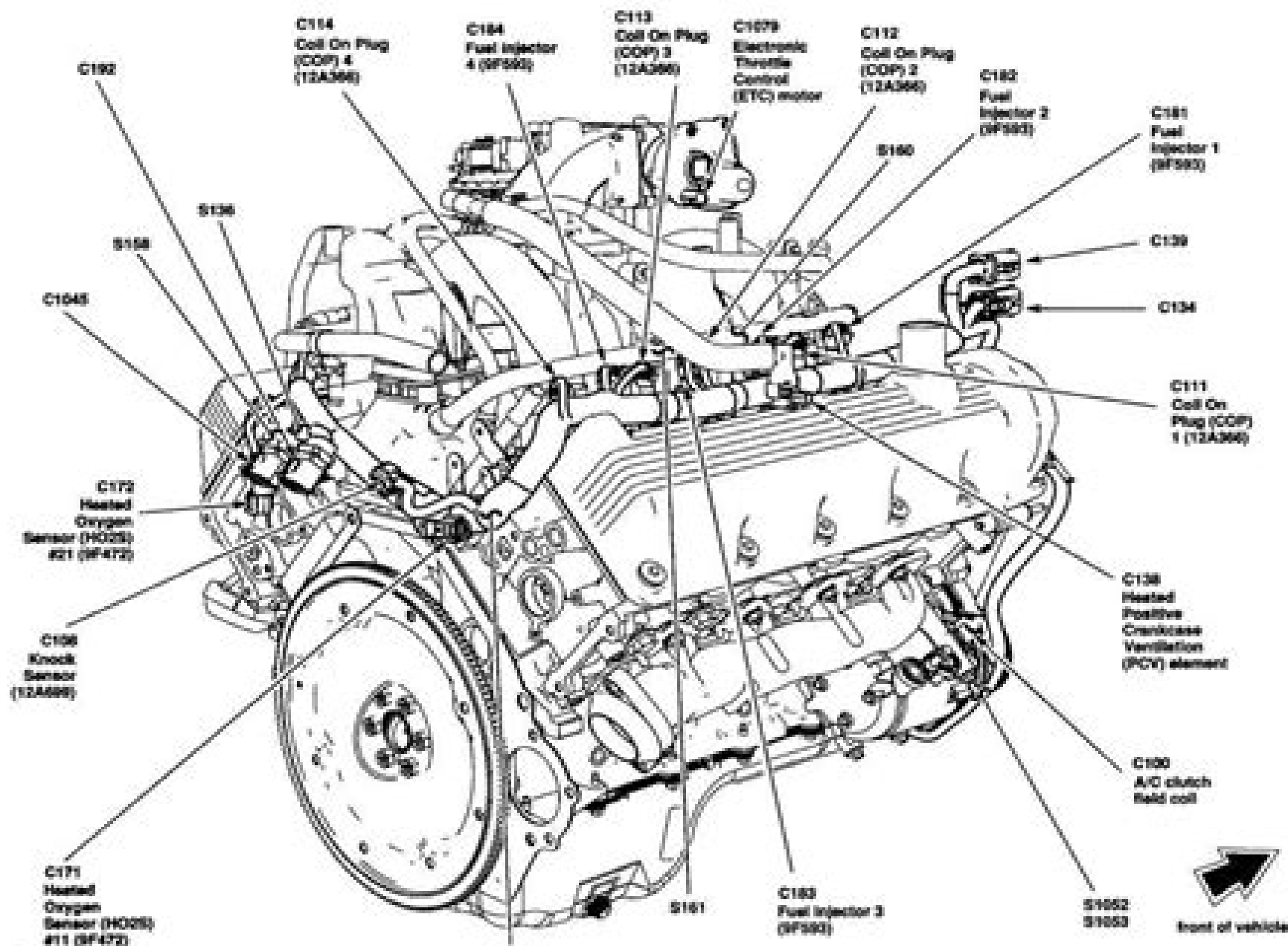
Fig. 9: Rear Of Engine (4.6L)
