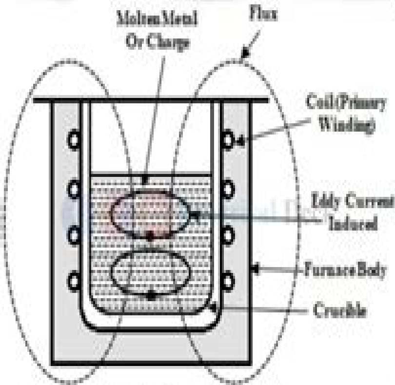
Coreless Induction Furnace
