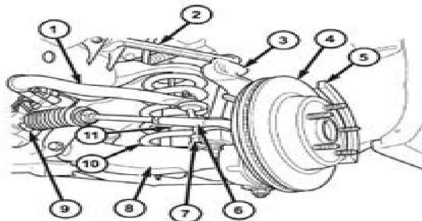
Fig. 1 FRONT SUSPENSION - 4X2
