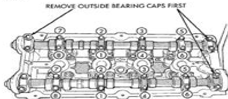
Fig. 23 Camshaft Bearing Cap— Removal
