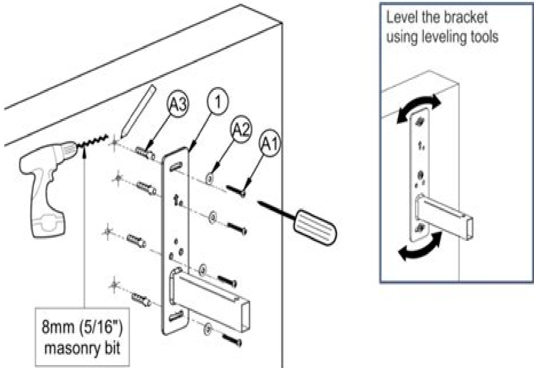
Figure 2: Attaching the Bracket to a Concrete Wall
