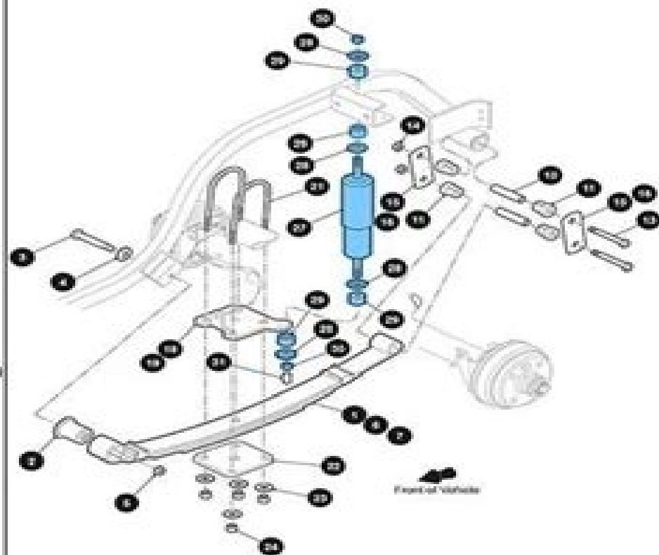
Rear Shock Absorbers (2pcs)
