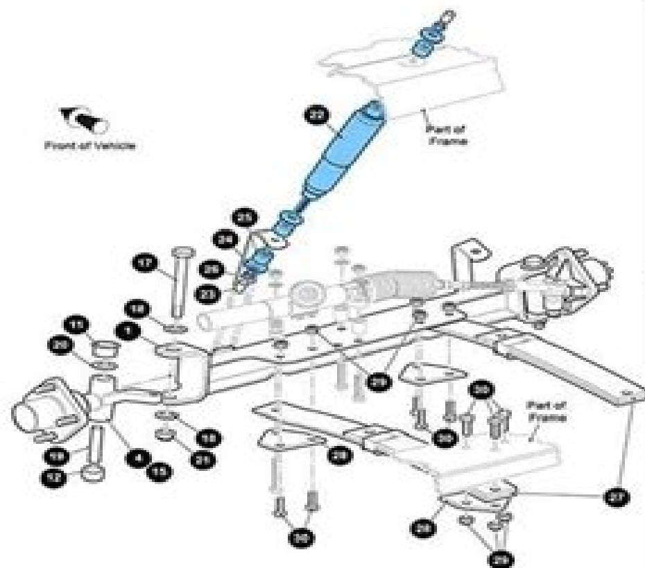
Front Shock Absorbers (2pcs)
